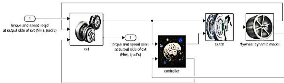
Figure 12. The contents of the mechanical hybrid system block
